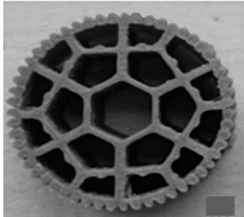
Figure S3. Cross-sectional plan of the K3 media
