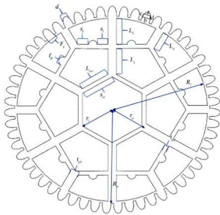
Figure S3. Cross-sectional plan of the K3 media
