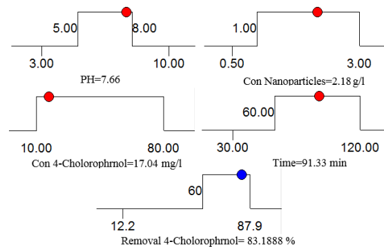
Figure S5. The optimal points of independent variables on the 4-CP removal rat by CCD-RSM model
