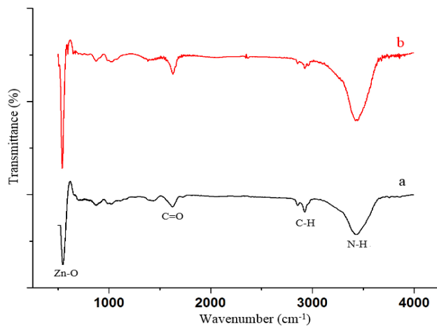
Figure S3. FTIR Diffractogram a) undoped ZnO b) MnO 3 - doped ZnO
