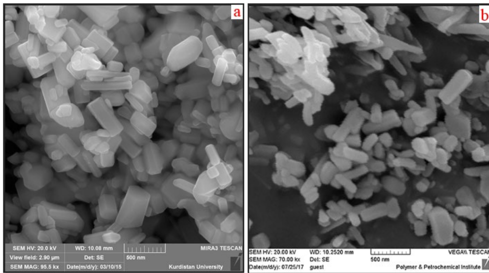
Figure S2. SEM Images of nanoparticles a) undoped ZnO b) 1% MnO 3 -doped ZnO
