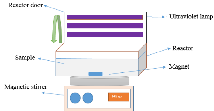
Figure S1. Schematic representation of photocatalytic reactor
