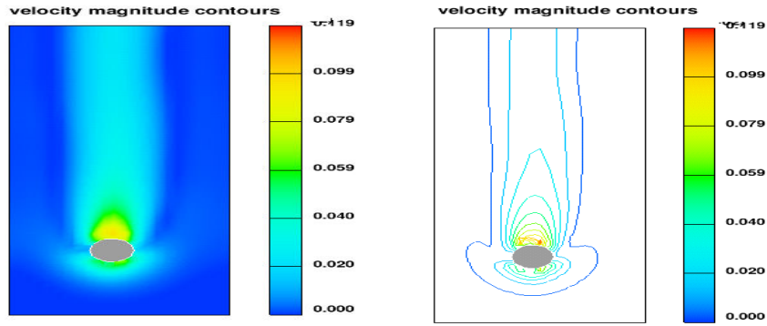
Fig. 2. Velocity magnitude contour of particle with diameter of 1.09 mm
