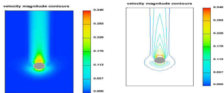
Fig. 4. Velocity magnitude contour of particle with diameter of 4.36 mm
