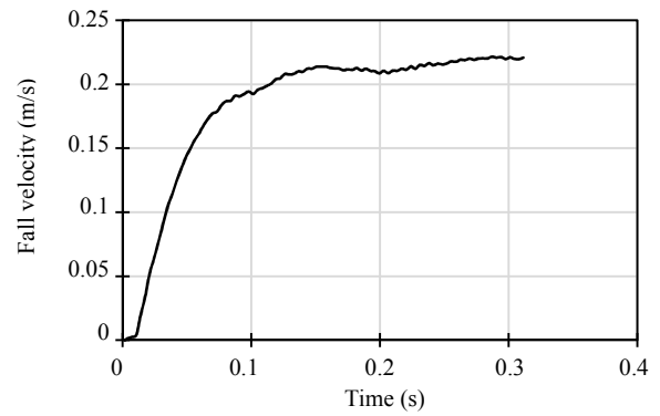
Fig. 6. Particle velocity versus time in particle with diameter of 1.09 mm
