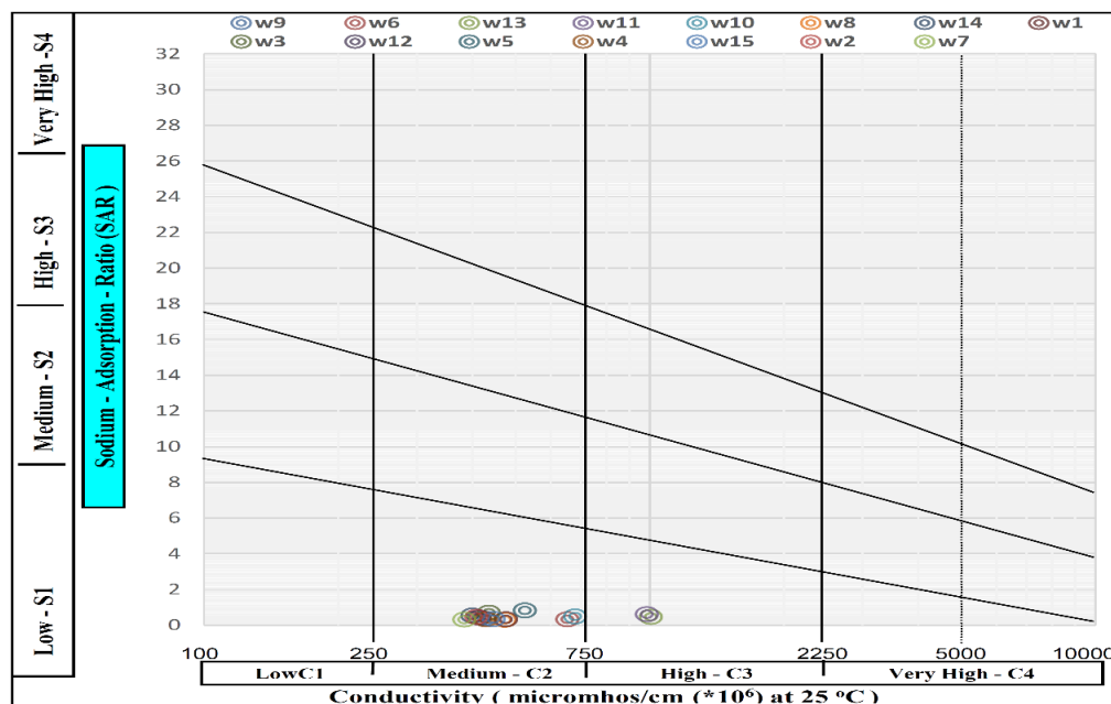
Fig. 3. Wilcox diagram
