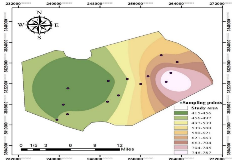
Fig. 4. Interpolation of EC values in Tuyserkan plain (micromhos/cm)
