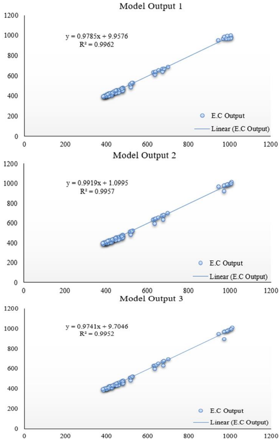
Fig. 5. Scatter plot of predicted and observed EC in models
