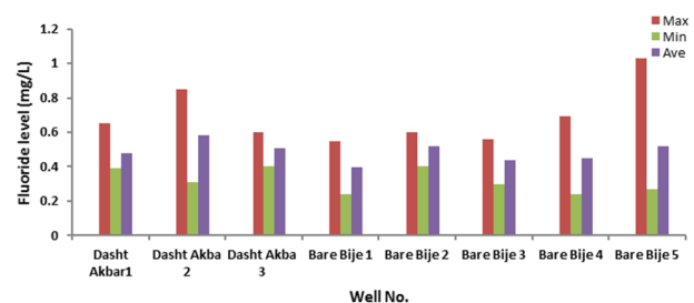
Fig.3 Average, maximum and minimum fluoride concentration(mg/l) of Dehloran drinking water sources in different months (a) and variety wells (b) in 2014
