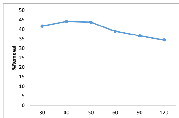
Figure 5. The removal efficiency of Cr (VI) by ferrous sulfate at different contact times (30, 40, 50, 60, 90, and 120 min)
