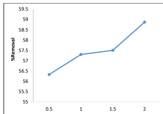
Figure 7. The removal efficiency Ni (II) by ferrous sulfate at different pH values
