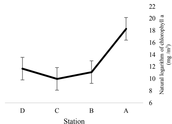
Fig. 2. Mean content of chlorophyll-a ( \text{mg}/\text{m}^3 ) in various stations in Choghakhor wetland (2017-2018)
