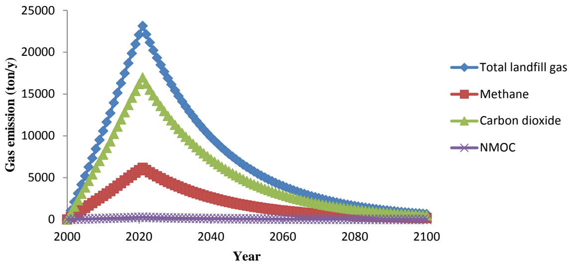
Figure 2. Annual landfill gas mass production provided by LandGEM models (2000-2100) in Sanandaj landfill k = 0.045 (/year), L_0 = 200 ( m^3 /ton), non-methane organic compound (NMOC) = 4000 ppmv, methane = 50%
