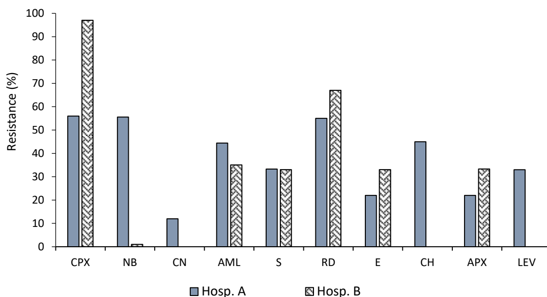
Fig. 2. Observed resistance in gram-positive bacterial isolates (CPX: ciprofloxacin, 10 µg; NB: norfloxacin, 10 µg; GN: gentamicin, 10 µg; AML: amoxil-amoxicillin, 20 µg; S: streptomycin, 30 µg; RD: rifampicin, 20 µg; E: erythromycin, 30 µg; CH: chloramphenicol, 30 µg; APX: ampiclox-ampicillin/cloxacillin, 20 µg; LEV: levofloxacin, 20 µg)
